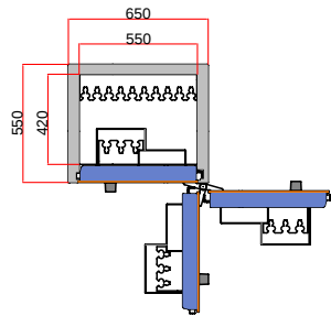
SWS / SWT 160/3-13
