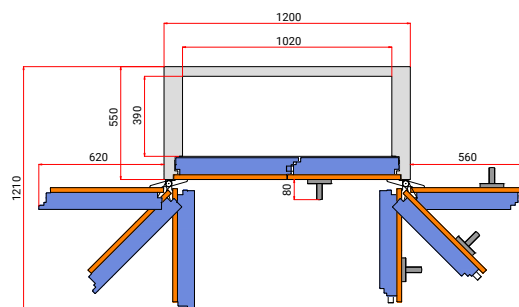
TSF 1012, 1912
