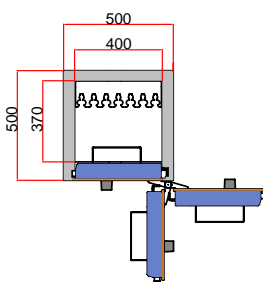
SWS / SWT 160/0-7
