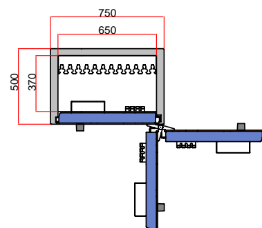
SWS / SWT 160/2-12
