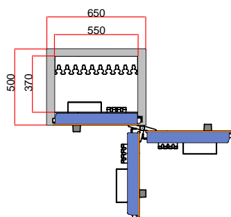
SWS / SWT 160/1-10
